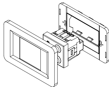
Figure 1: Montage Rectangulaire + Monture
